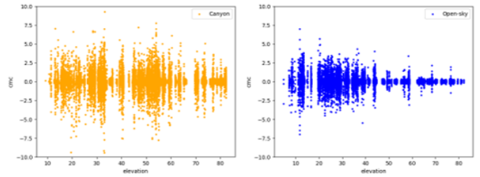
Fig. 4. CMC variations of LOS satellites in an urban canyon and in an open sky area.
