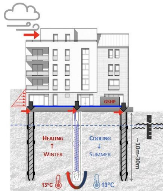
Figure 1. Combined loads acting on energy piles.
