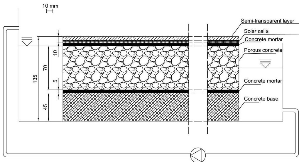
Figure 1: Sketch of the laboratory prototype (in mm)
