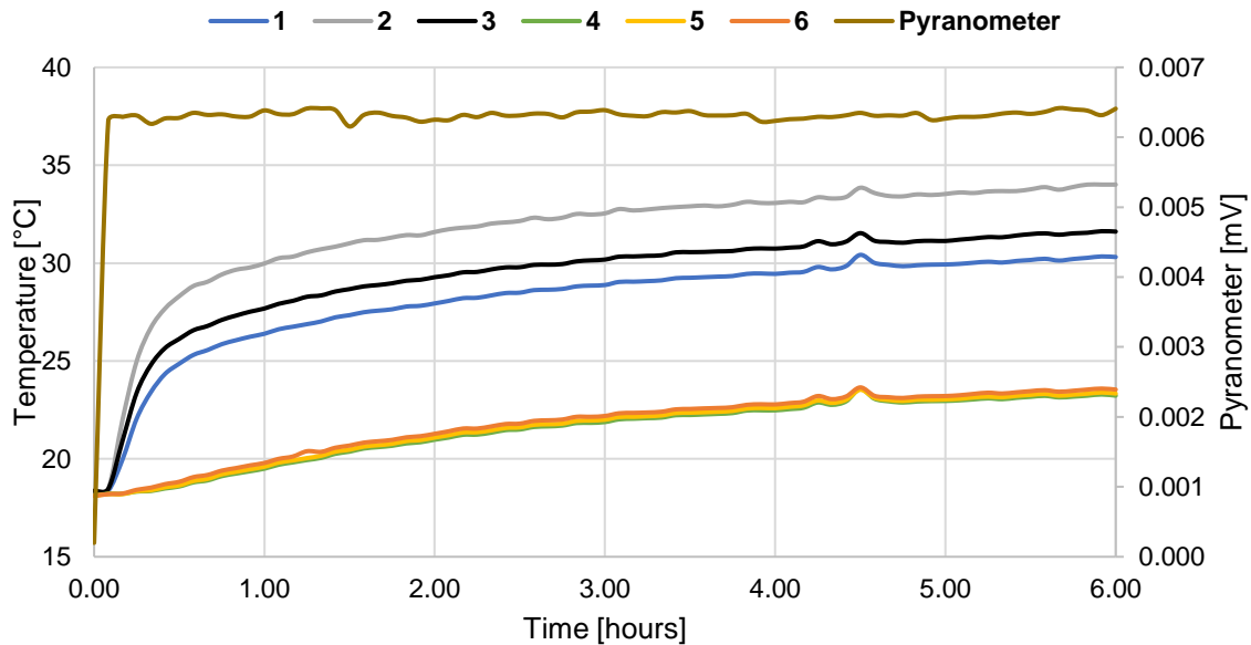
Figure 5: Experimental temperature variations in presence of water flow
