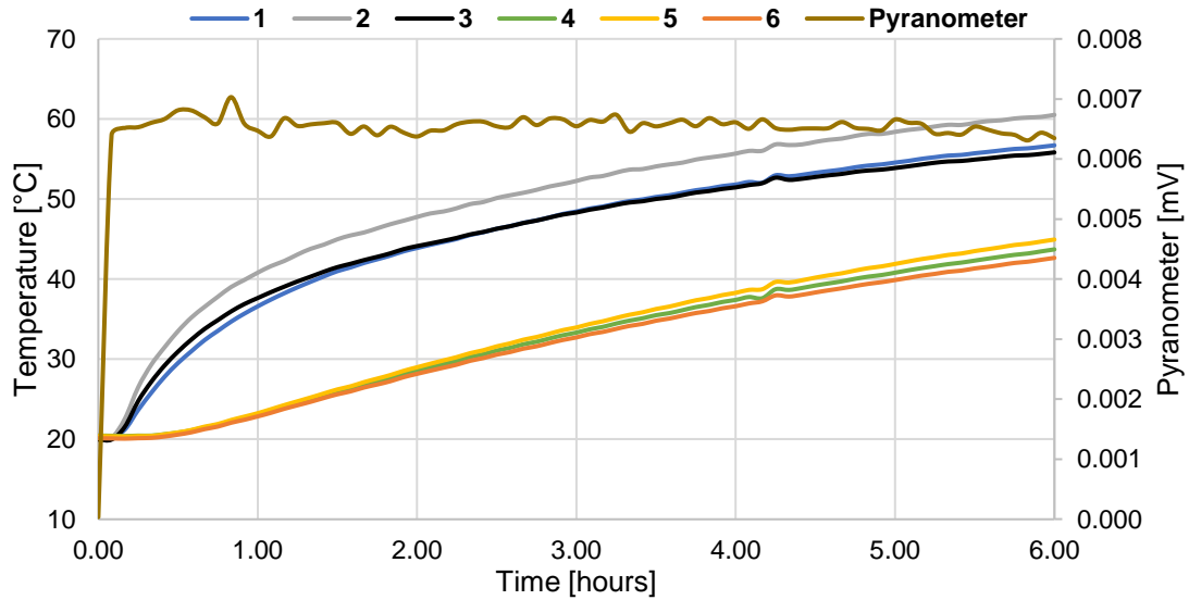
Figure 4: Experimental temperature variations in absence of water flow
