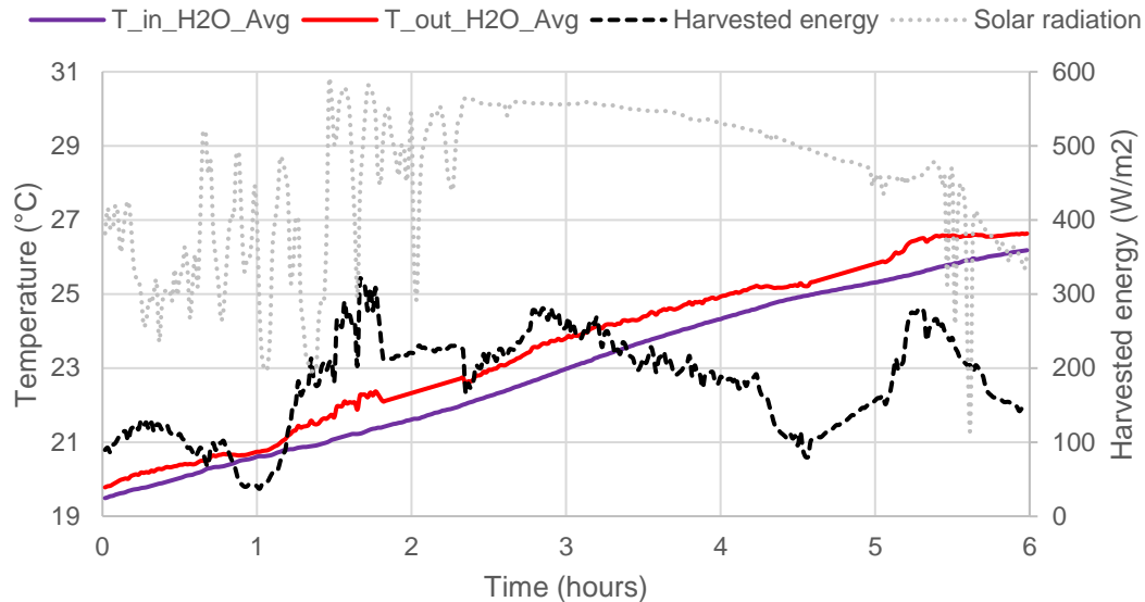
Figure 7: Example of harvested energy by the porous concrete in the full-scale prototype in outdoor conditions
