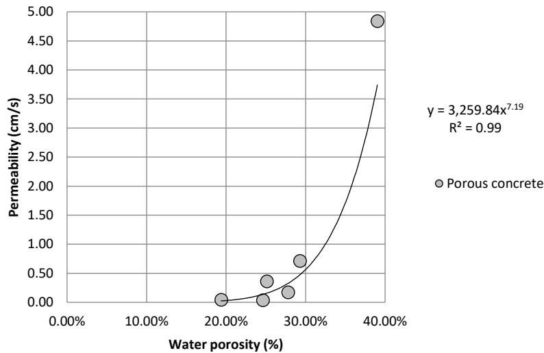
Figure 2: Permeability vs porosity
