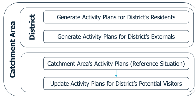
Figure 2. Overview of the proposed approach to generate activity plans in the projected situation at the district and catchment area levels. The activity plans of district residents and externals are first generated. In parallel, the activity plans of the agents in the catchment area are generated in a similar way to the reference situation, while for potential visitors, new plans will be included with a secondary activity performed in the district.
