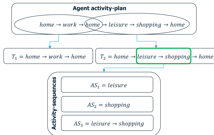
Figure 11. Potential visitor’s activity plan and its derived activity sequences. The given activity plan is divided into two tours: T_1 with work activity and T_2 with sequence of leisure and shopping activities. From T_2 , three sequences of activities AS can take place in LaVallée, which are (1) leisure, (2) shopping, and (3) leisure followed by shopping.
