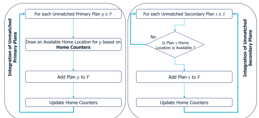
Figure 6. Integration of unmatched plans. Primary and secondary plans are sequentially integrated in the final set of plans. The primary plans are the first ones inserted, which depend on the constraints of the study, for instance, a known number of inhabitants per home location.
