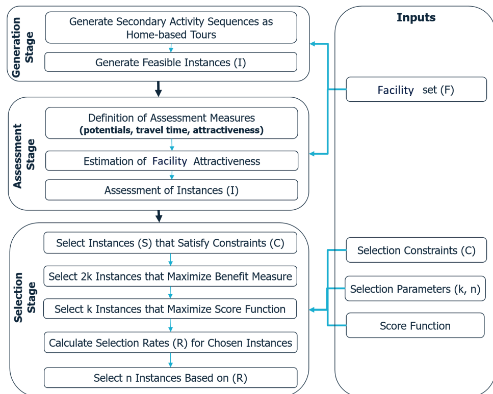
Figure 4. A detailed view of the location-choice process. It consists of a set of inputs and three main stages. In the generation stage, all home-based tours with at least one secondary activity are first generated
