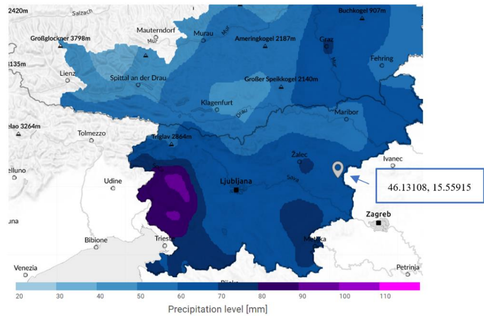
Figure 2. Map of extreme precipitation level with return period of 100 years. The location of a selected landslide is plotted [50].
