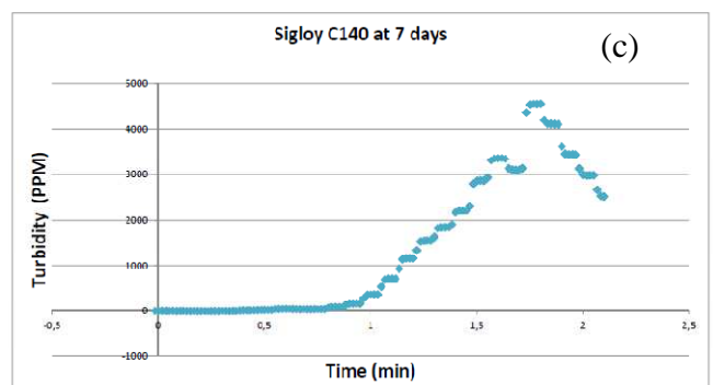
Turbidity (PPM) vs Time (min)
