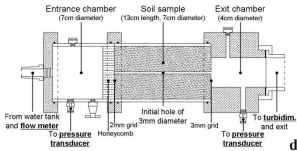
Figure 2. Hole erosion test set-up. (a) Image of eroding unit. (b) Sample before test with 3mm diameter hole. (c) Cut sample after test with molded wax. (d) Drawing of eroding unit. Sensors are indicated in bold and underlined characters.
