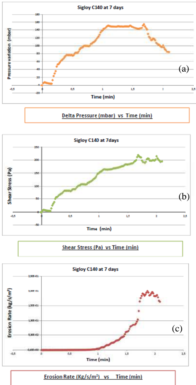
Figure 4. Hole erosion test set-up. (a) variation of pressure, (b) shear stress vs time, (c) erosion rate vs time.
