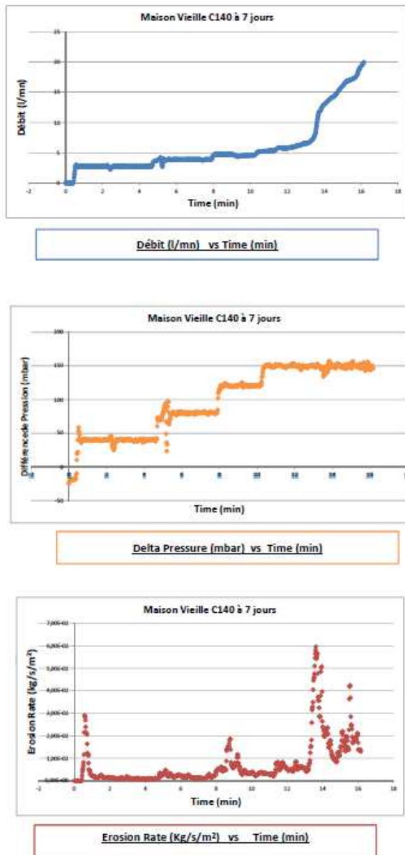
Figure 6. Hole erosion test set-up. (a) Flow, (b) variation of pressure vs time, (c) erosion rate vs time
