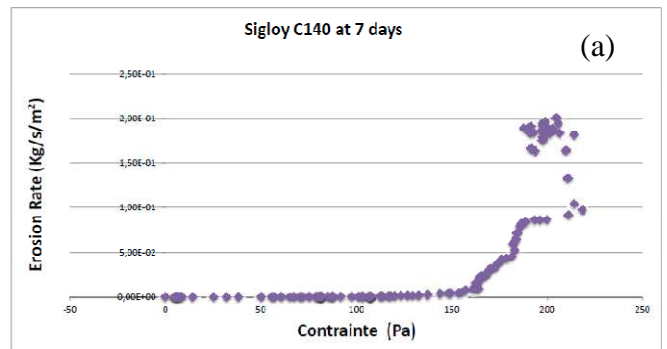
Erosion Rate (Kg/s/m 2 ) vs Conainte (Pa)
