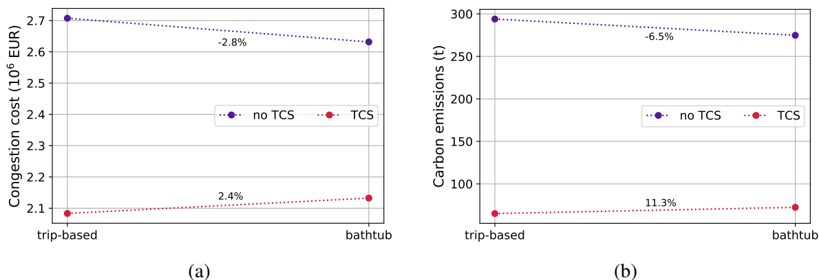
FIGURE 10: Variations of the objectives measures between bathtub and trip-based MFD: (a) congestion cost (total schedule cost) and (b) carbon emission.
