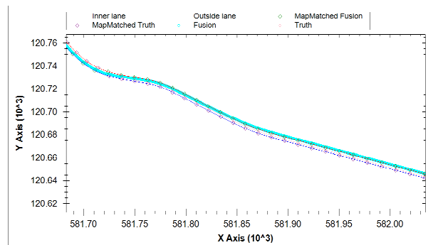
Figure 8: No-EGNOS area with system B
