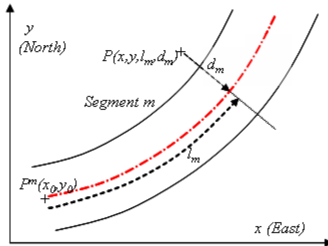
Figure 2 – Dual representation of the vehicle position in East, North and the segment reference.
