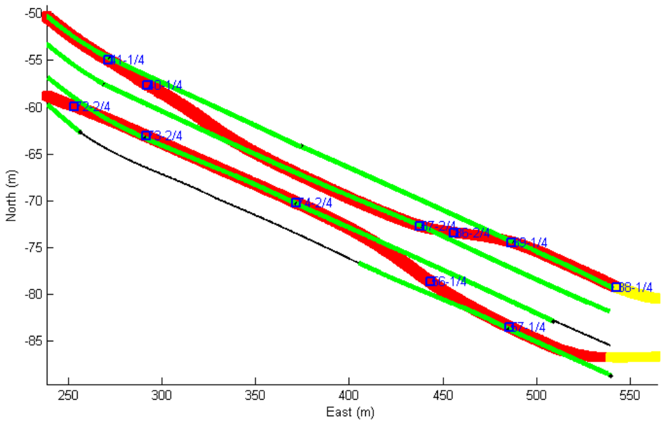
Figure 3 – Results of the combined GNSS/DR/Emap algorithm. Solid black: map representation of the road. Solid green: segment to which the vehicle is assigned in the map-matching process (end of segment is noted with a black dot). Red square: filter position output within the Emap. Yellow square: filter position output out of the Emap bounds. Blue square: positions where the vehicle changes the lane as provided by the algorithm. Next to the blue square, the identifier of the new lane and its relative lateral position in the carriageway are shown.
