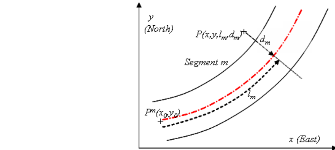
Figure 2 – Dual representation of the vehicle position in East, North and the segment reference.
