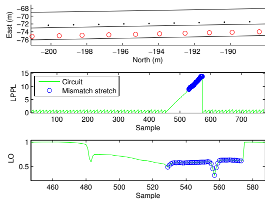
Fig. 5. (Top) A stretch of estimated vehicle trajectory during a mismatch: road lanes (solid black), ground truth (black ·), filter positions (red o). (Middle) LPPL values along a stretch of the circuit (solid green) and during the period of mismatch (blue o). (Bottom) \mu LO values along a stretch of the circuit (solid green) and during the period of mismatch (blue o).
