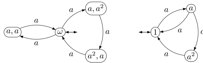
■ Figure 3 The flower automaton and the prefix automaton of X (Example 4).
