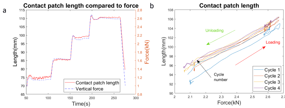
Fig. 7 (a) Contact patch length comparison with vertical force actuator command; (b) Contact patch length variation through cycles
