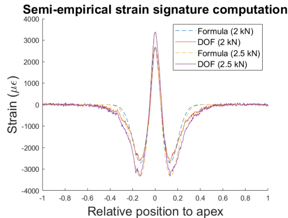
Fig. 9 Comparison of the semi empirical model (dashed curves) with the DOF measurement for 2 vertical forces
