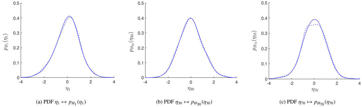
Figure 9: Scenario 2: probability density functions of components H_1 , H_{30} , and H_{70} of \mathbf{H} , estimated with the training dataset (dashed line) and with the learned dataset (solid line).
