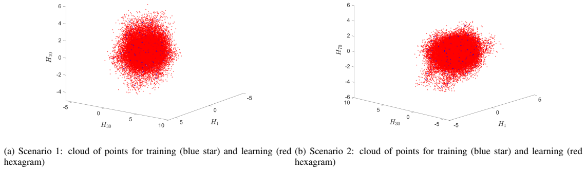
Figure 10: Clouds of the learned points and the training points of \mathbf{H} , associated with components H_1 , H_{30} , and H_{70} .
