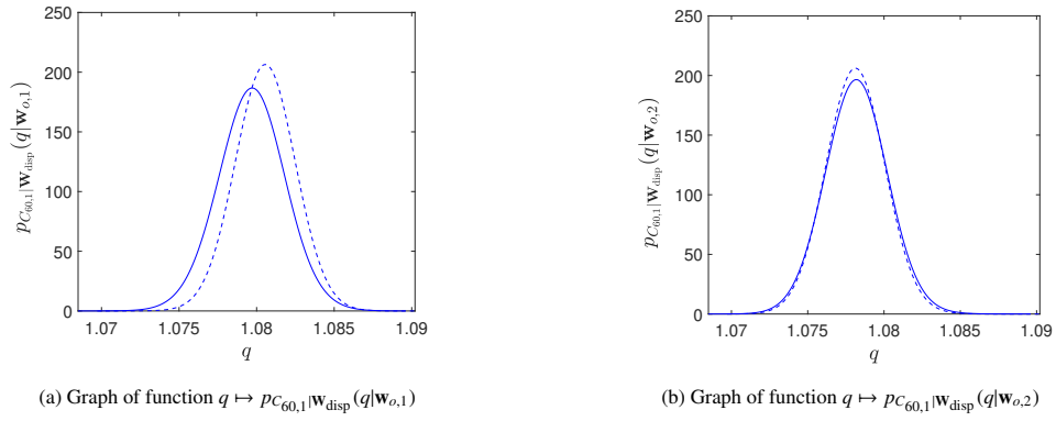
Figure 14: Validation of Scenario 2: Graph of the conditional pdf given \mathbf{W}_{\text{disp}} = \mathbf{w}_{0,1} or \mathbf{w}_{0,2} of component 1 of the random tensor \mathbf{C} at point 60. Learned dataset (solid line), validation dataset (dashed line).
