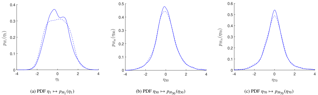
Figure 8: Scenario 1: probability density functions of components H_1 , H_{30} , and H_{70} of \mathbf{H} , estimated with the training dataset (dashed line) and with the learned dataset (solid line).
