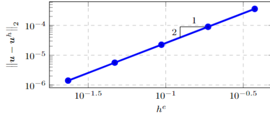
Figure 3: Convergence of the L^2 error ( h -refinement) for the reference solution.
