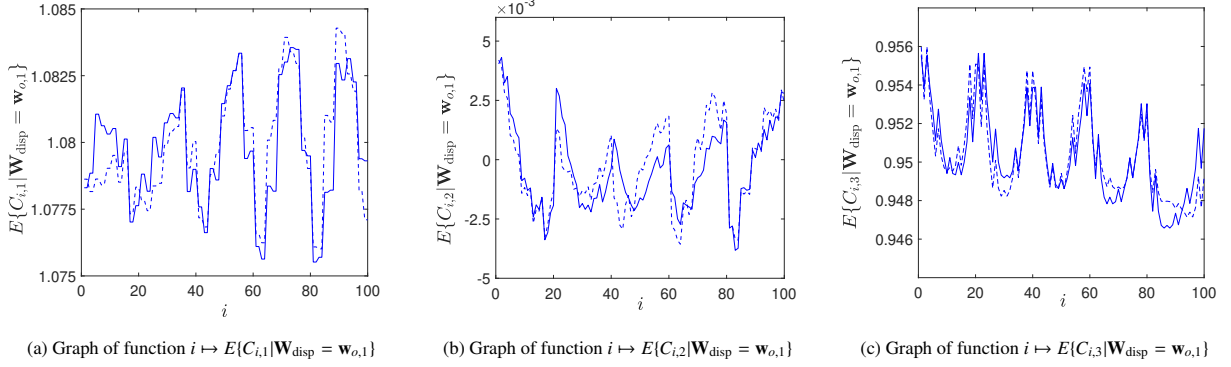
Figure 16: Validation of Scenario 2: Graph of the conditional mathematical expectation as function of points i given \mathbf{W}_{\text{disp}} = \mathbf{w}_{o,1} for the three components of the random tensor \mathbf{C} . Learned dataset (solid line), validation dataset (dashed line).
