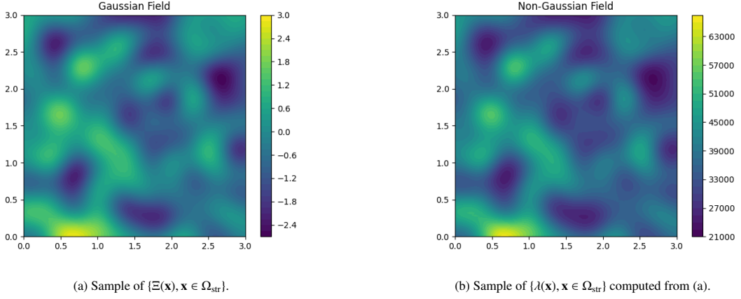
Figure 2: Realizations of the underlying Gaussian field (left) and material parameter random field (right).
