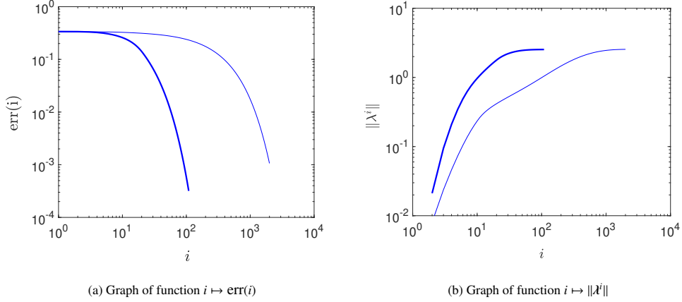
Figure 7: Convergence analysis of the iterative algorithm to take into account the constraints on second-order moments of \mathbf{H} in PLoM as a function of iteration number i , presented in log-log scales. Scenario 1 (thin line), Scenario 2 (thick line).
