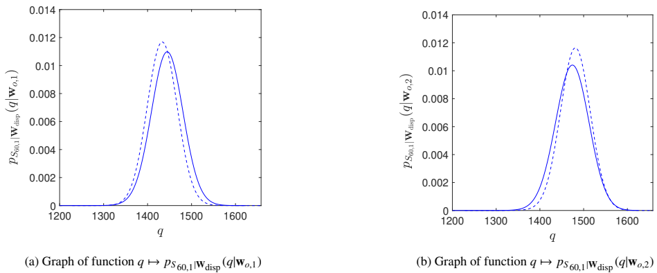
Figure 15: Validation of Scenario 2: Graph of the conditional pdf given \mathbf{W}_{\text{disp}} = \mathbf{w}_{0,1} or \mathbf{w}_{0,2} of component 1 of the random tensor \mathbf{S} at point 60. Learned dataset (solid line), validation dataset (dashed line).
