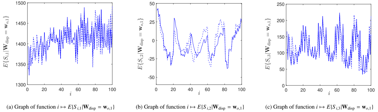
Figure 18: Validation of Scenario 2: Graph of the conditional mathematical expectation as function of points i given \mathbf{W}_{\text{disp}} = \mathbf{w}_{o,1} for the three components of the random tensor \mathbf{S} . Learned dataset (solid line), validation dataset (dashed line).
