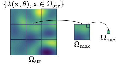
Figure 1: Definition of scales in the concurrent multiscale simulations. Fluctuations in the first Lamé parameter \lambda are introduced at fine scale.
