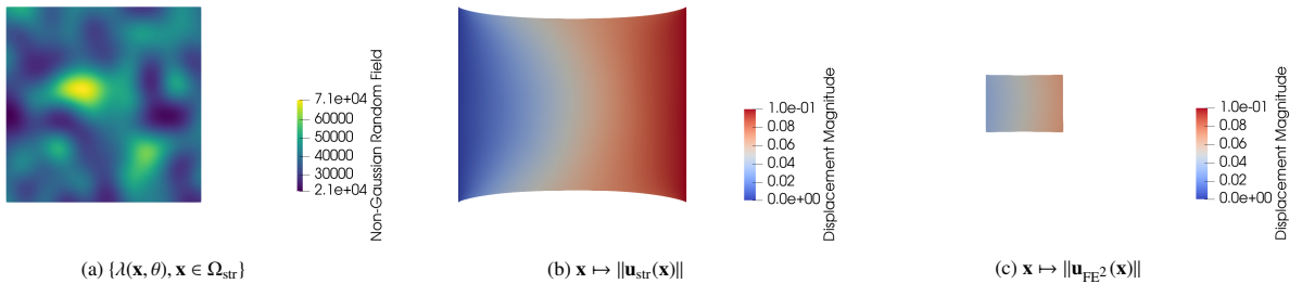
Figure 4: Sample of the material parameter \lambda (left) and associated displacement magnitudes for the solutions on \Omega_{\text{str}} (middle) and \Omega_{\text{mac}} (right).
