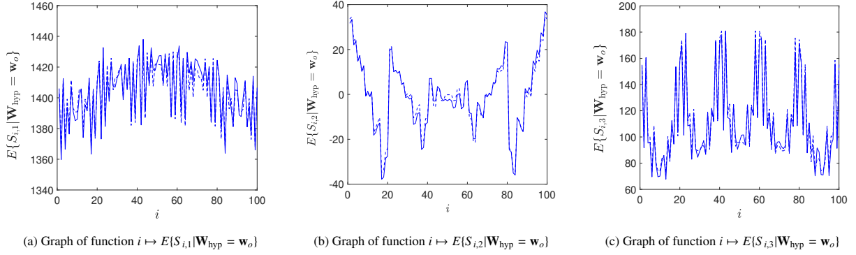
Figure 13: Validation of Scenario 1: Graph of the conditional mathematical expectation as function of points i given \mathbf{W}_{\text{hyp}} = \mathbf{w}_0 for the three components of the random tensor \mathbf{S} . Learned dataset (solid line), validation dataset (dashed line).
