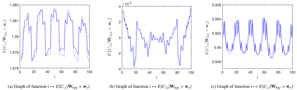
Figure 12: Validation of Scenario 1: Graph of the conditional mathematical expectation as function of points i given \mathbf{W}_{\text{hyp}} = \mathbf{w}_o for the three components of the random tensor \mathbf{C} . Learned dataset (solid line), validation dataset (dashed line).
