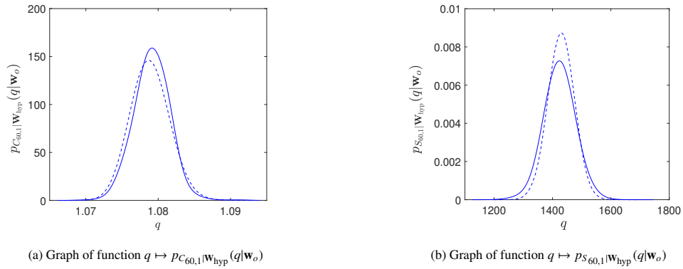
Figure 11: Validation of Scenario 1: Graph of the conditional pdf given \mathbf{W}_{\text{hyp}} = \mathbf{w}_o of component 1 of the random tensors \mathbf{C} and \mathbf{S} at point 60. Learned dataset (solid line), validation dataset (dashed line).
