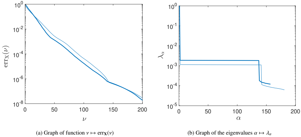
Figure 6: Convergence of the PCA reduced representation (a). Eigenvalues of the transition matrix [\mathbb{P}] for the diffusion-maps basis (b). Scenario 1 (thin line), Scenario 2 (thick line).
