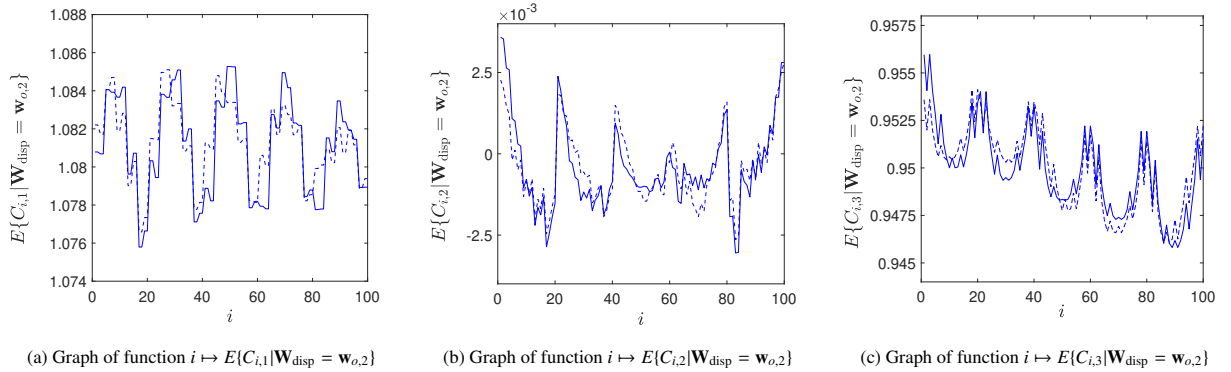
Figure 17: Validation of Scenario 2: Graph of the conditional mathematical expectation as function of points i given \mathbf{W}_{\text{disp}} = \mathbf{w}_{o,2} for the three components of the random tensor \mathbf{C} . Learned dataset (solid line), validation dataset (dashed line).
