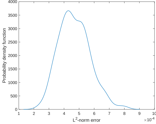
Figure 5: Probability density function of the normalized L^2 -norm error (estimated with 500 samples).
