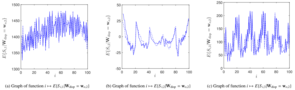
Figure 19: Validation of Scenario 2: Graph of the conditional mathematical expectation as function of points i given \mathbf{W}_{\text{disp}} = \mathbf{w}_{o,2} for the three components of the random tensor \mathbf{S} . Learned dataset (solid line), validation dataset (dashed line).
