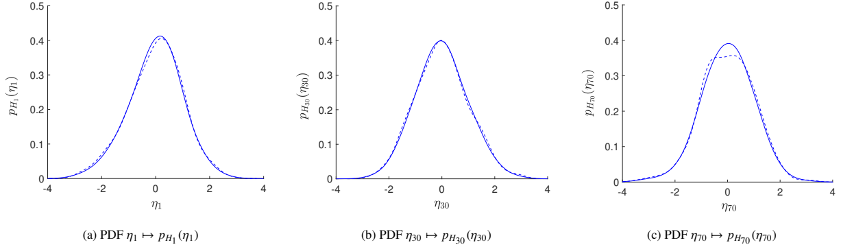
Figure 9: Scenario 2: probability density functions of components H_1 , H_{30} , and H_{70} of \mathbf{H} , estimated with the training dataset (dashed line) and with the learned dataset (solid line).
