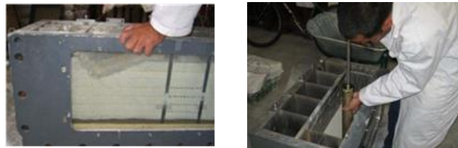
Figure 49 Preparation of a test of wetting-induced collapse in embankment base
