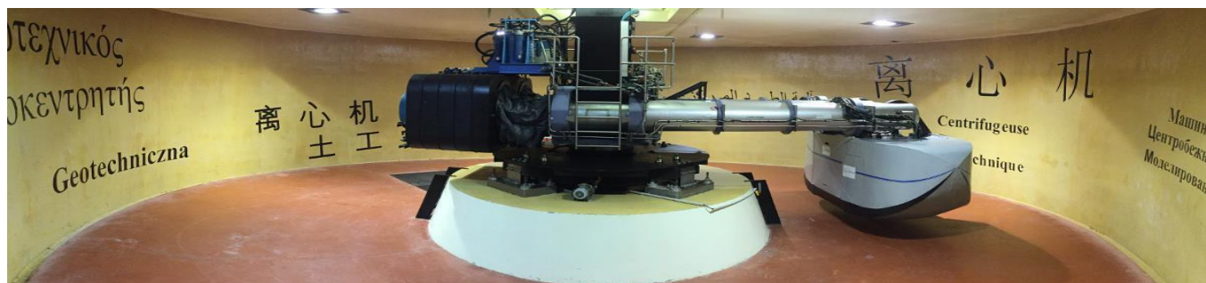
Figure 44 The 200xg-ton Centrif-UGE (5.5m radius)
