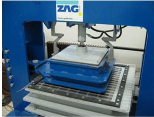
Figure 4 Loading frame when direct shear mode is used
