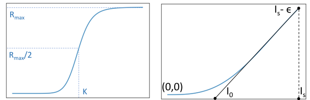
Fig. 2: Left: the Naka-Rushton function with parameters R_{max} , K and n . Right: the modulation function, shaped like the lefthand side of the Naka-Rushton function, showing parameters I_s , I_0 and \epsilon .
