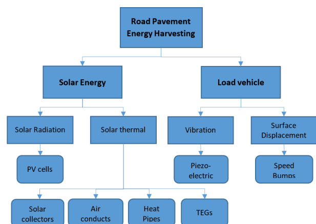
Figure 1. Energy harvesting through the road pavement.
