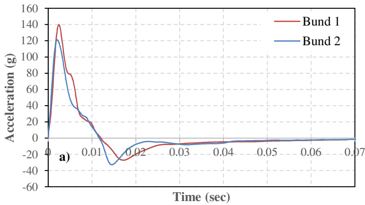
262 263 Figure 8. a) Acceleration of acc3 sensor for both embankments and b) position of the sensors in plan view
