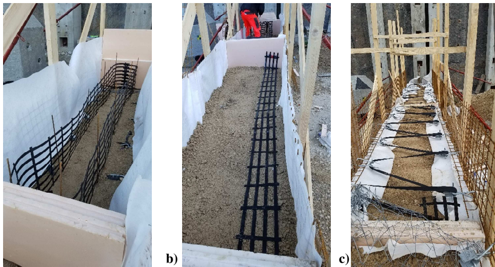
166 a) 167 b) 168 Figure 3. Construction of a) Embankment 1, b) Embankment 2 and c) facing retaining system for both embankments
