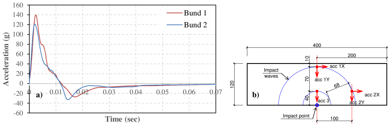
262 263 Figure 8. a) Acceleration of acc3 sensor for both embankments and b) position of the sensors in plan view
