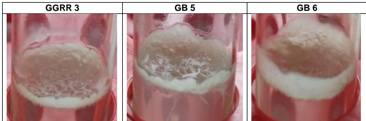
Figure 5. Microorganisms in nutrient liquid media pH 11. GGRR 3 is the colony number three isolated from the GGRR granulate, GB 5 AND GB 6 are MO isolated from the GB granulate.
