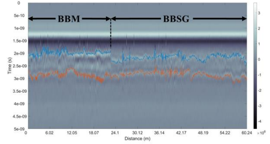
Fig. 6. Example of a B-Scan representing the longitudinal profile P3 with the bottom of the wearing course in blue and the bottom of the binder course in orange
