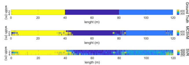
Fig. 10. a) Ground truth distinguishing 3 zones, 450 g/m² in yellow, 250 g/m² in dark blue and 350 g/m² in light blue b) Classification mapping based on MCSVM applied to GPR data c) Regression mapping (estimated values) based on SVR applied to GPR data
