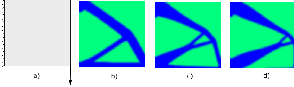
Figure 1: a) The Design domain, boundary conditions, external load for optimization of a cantilever beam. b) The optimised solution for the homogeneous material, c) optimised solution for FGM with \frac{E_1}{E_2} = 50 with z = 2 , and d) optimised solution for FGM with z = 4 .
