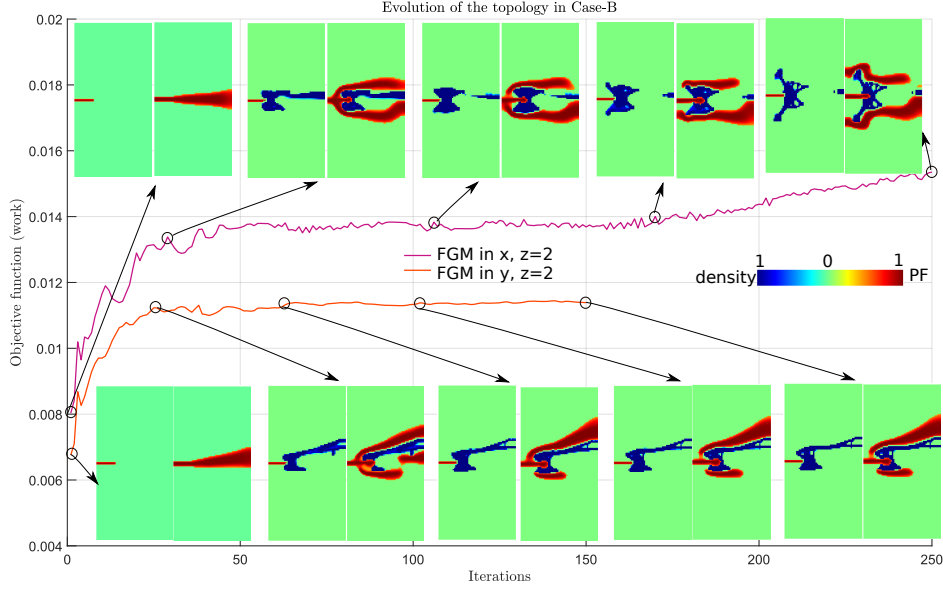
Figure 9: Evolution of the optimum topology in Case-B for the grading in X-direction and Y-direction for the volume fraction of 5% and z = 2 in y-direction for 5 percent volume fraction of inclusion
