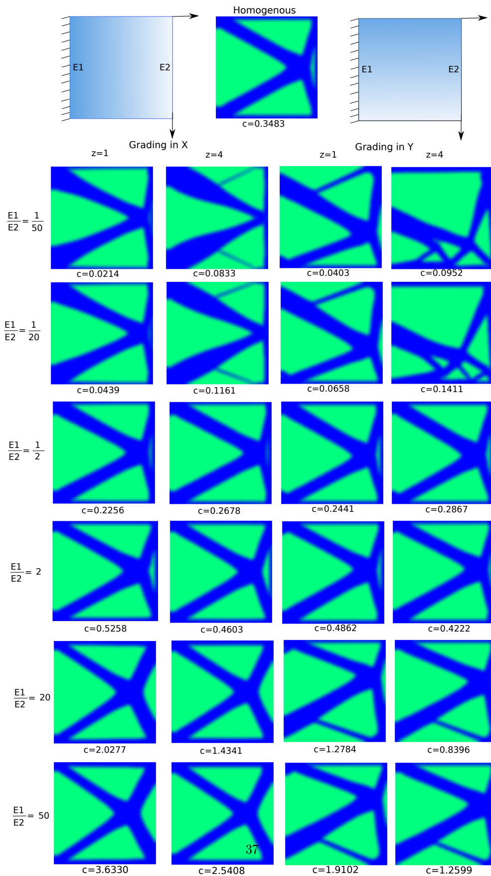
Figure 23: The Design domain, boundary conditions, external load for optimization of a cantilever beam with two load cases, and the optimized design for FGM with grading in x-direction and y-direction (separately) for different grading profiles.
