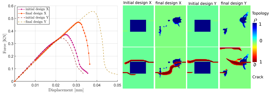
Figure 20: a) Force Vs. displacement with improved performance for Case-B, and b) Final optimum solution from the initial design along with the corresponding crack propagation.
