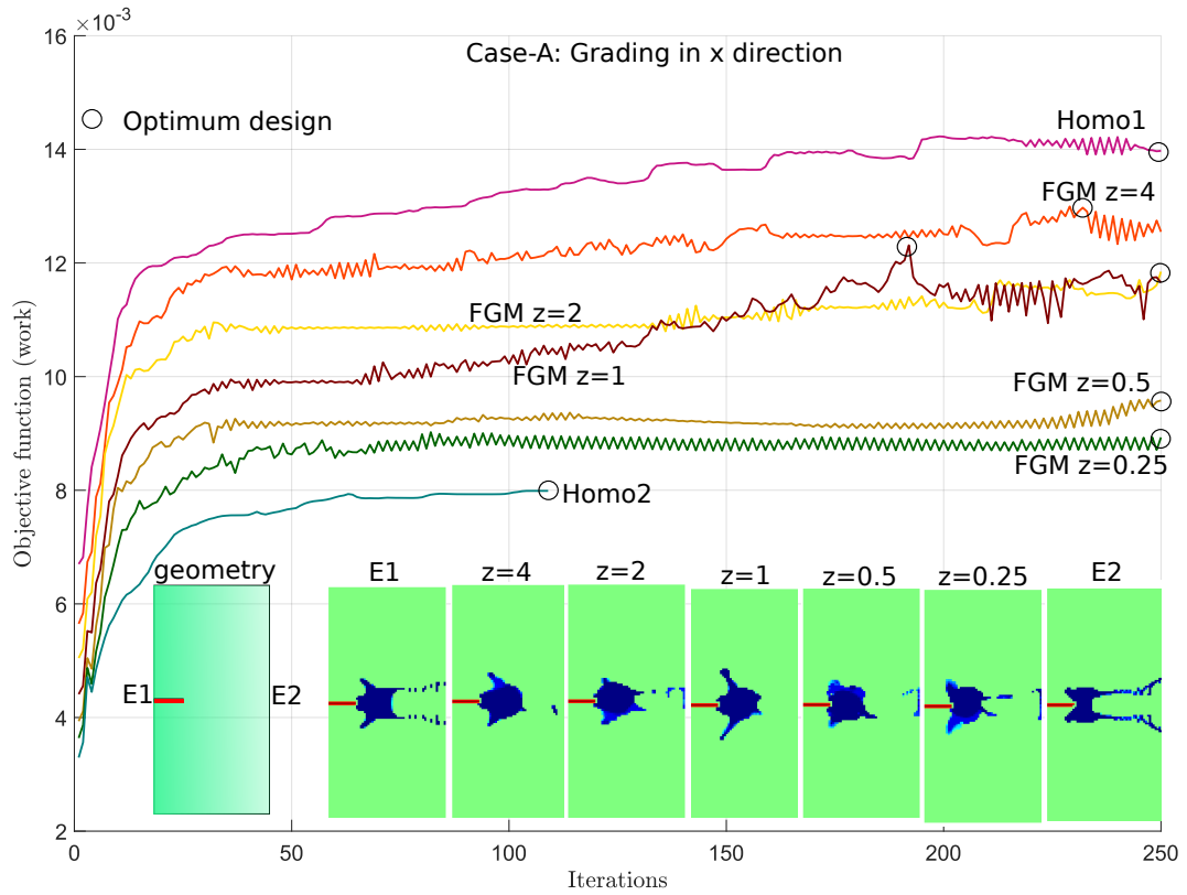
Figure 4: Grading in the x-direction for 5 percent volume fraction of inclusion for Case-A
