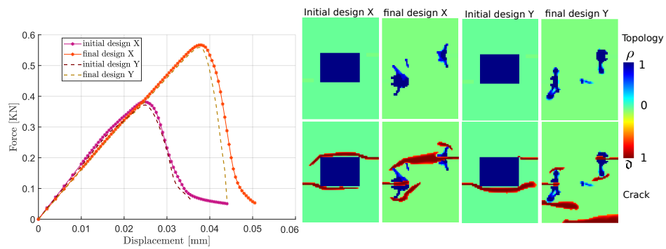
Figure 19: a) Force Vs. displacement with improved performance for Case-A, and b) Final optimum solution from the initial design along with the corresponding crack propagation.
