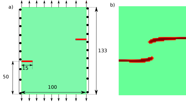
Figure 14: a) geometrical description of the asymmetrical notched specimen, b) crack propagation in the asymmetrical notch for homogeneous material medium.
