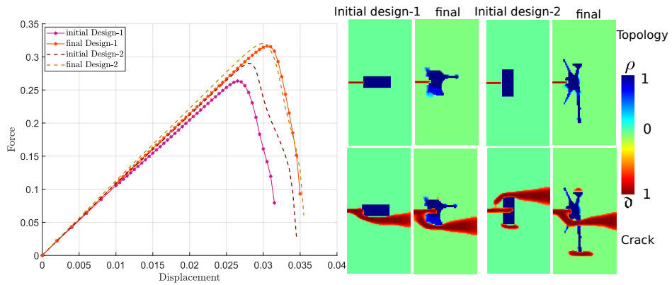
Figure 13: a) Force Vs. displacement of Design-1 and Design-2 with improved performance for Case-B, for grading in the x-direction, and b) Final optimum solution from the initial design along with the corresponding crack propagation.
