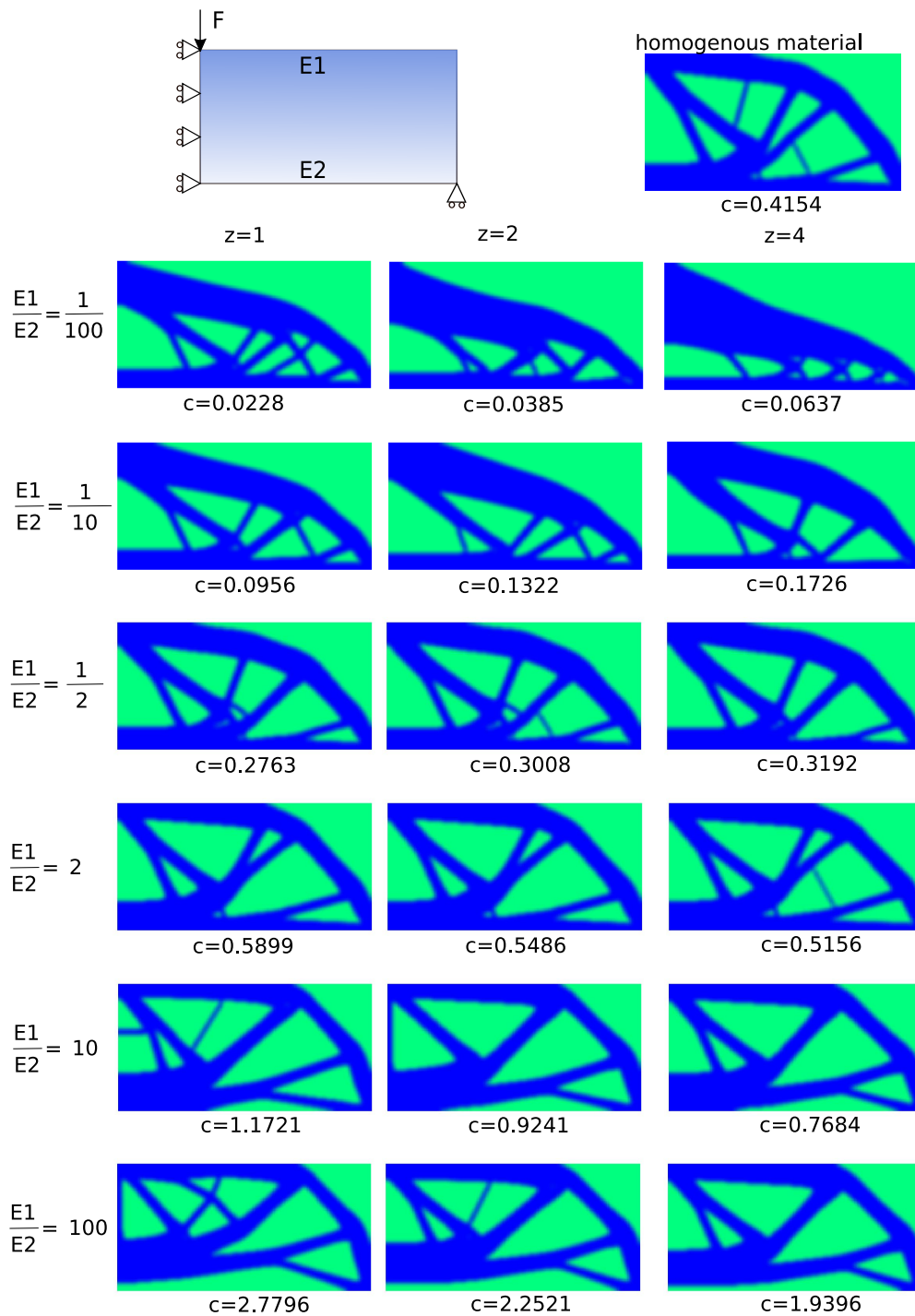
Figure 3: The Design domain, boundary conditions, external load for optimisation of a symmetric MBB beam along with the optimised design for FGM with grading in y -direction for different grading profiles.
