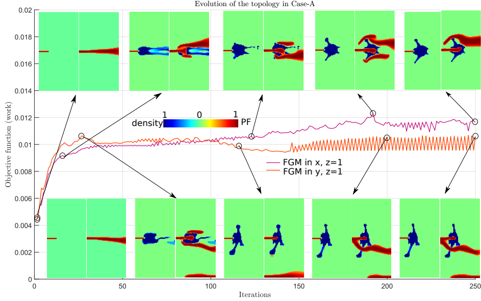
Figure 6: Evolution of the optimum topology in Case-A for the grading in X-direction and Y-direction for the volume fraction of 5% and z = 1 in y-direction for 5 percent volume fraction of inclusion.
