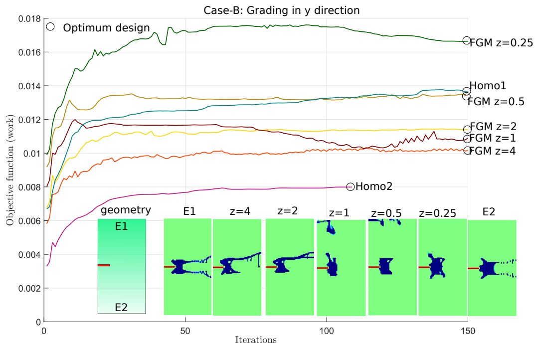
Figure 8: Grading in the y-direction for 5 percent volume fraction of inclusion for Case-B
