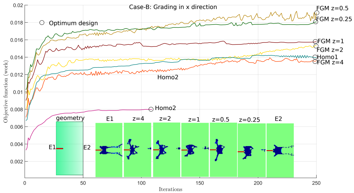
Figure 7: Grading in the x-direction for 5 percent volume fraction of inclusion for Case-B
