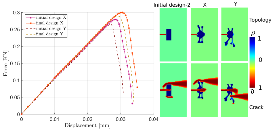
Figure 12: a) Force Vs. displacement of Design-2 with improved performance for Case-A, and b) the final optimum solution from the initial design along with the corresponding crack propagation.
