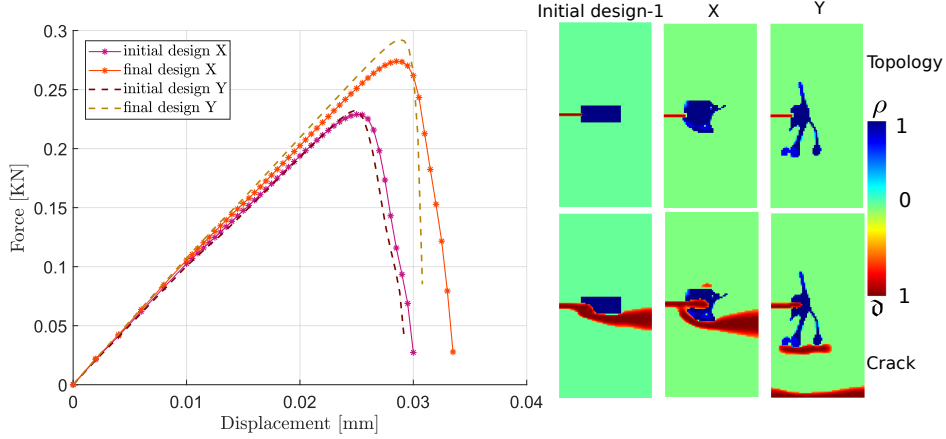
Figure 11: a) Force Vs. displacement of Design-1 with improved performance for Case-A, and b) the final optimum solution from the initial design along with the corresponding crack propagation.
