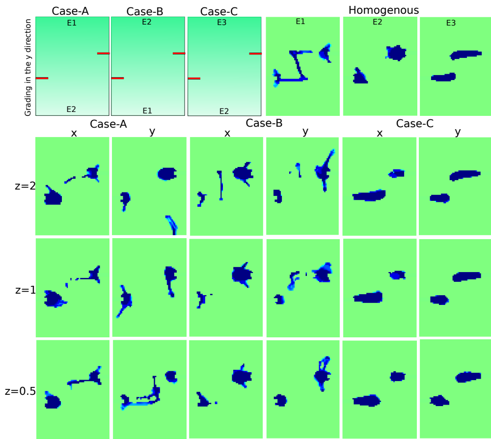
Figure 18: Overview of the optimum topologies for volume fraction of 5% for different cases and different z with E1 = 5.2 , E2 = 10.4 , and E3 = 20.8
