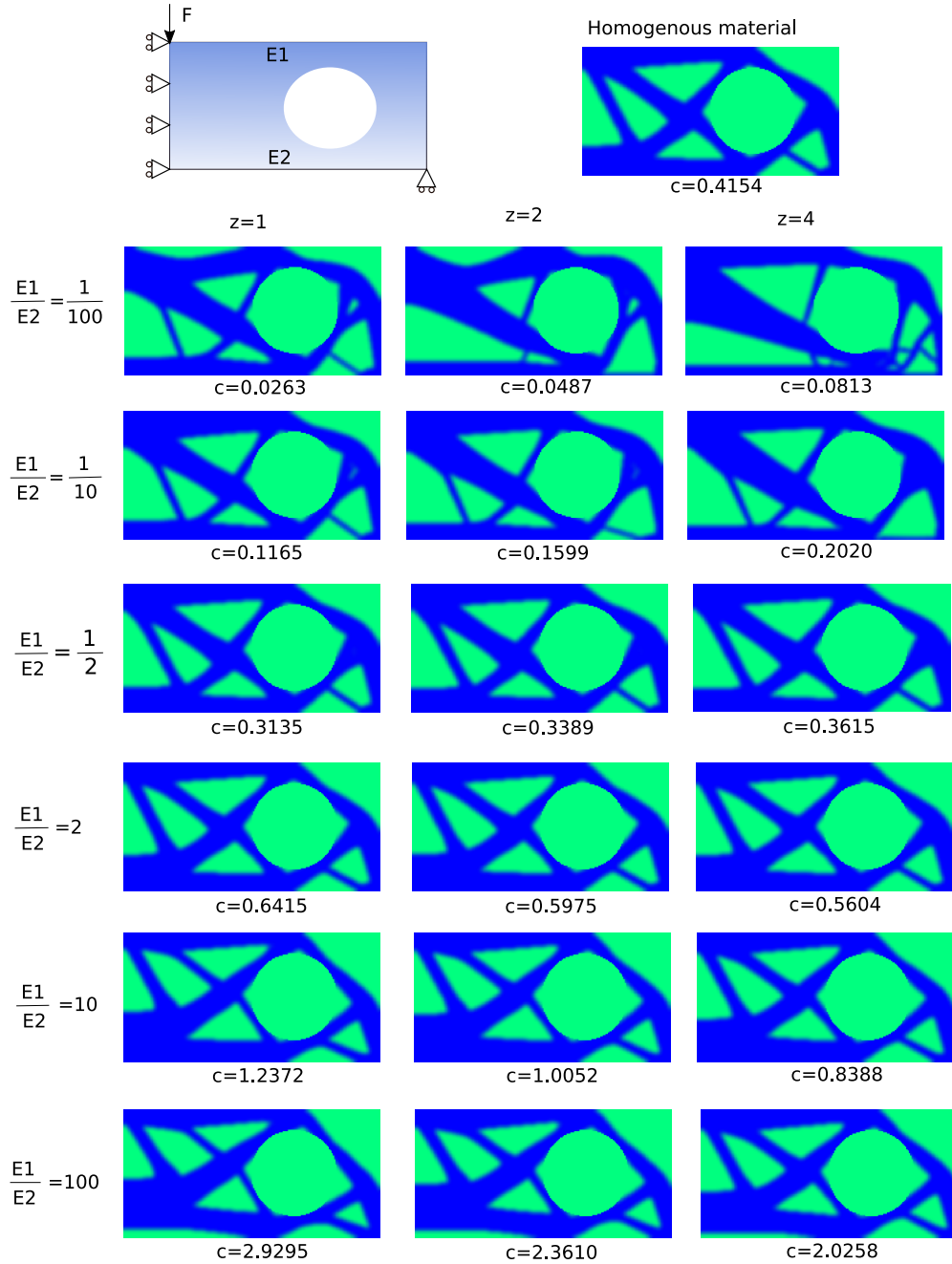
Figure 22: The Design domain, boundary conditions, external load for optimization of a symmetric MBB beam with a hole along with the optimized design for FGM with grading in y-direction for different grading profiles.
