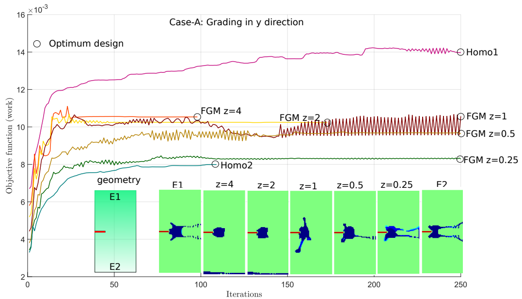
Figure 5: Grading in the y-direction for 5 percent volume fraction of inclusion for Case-A
