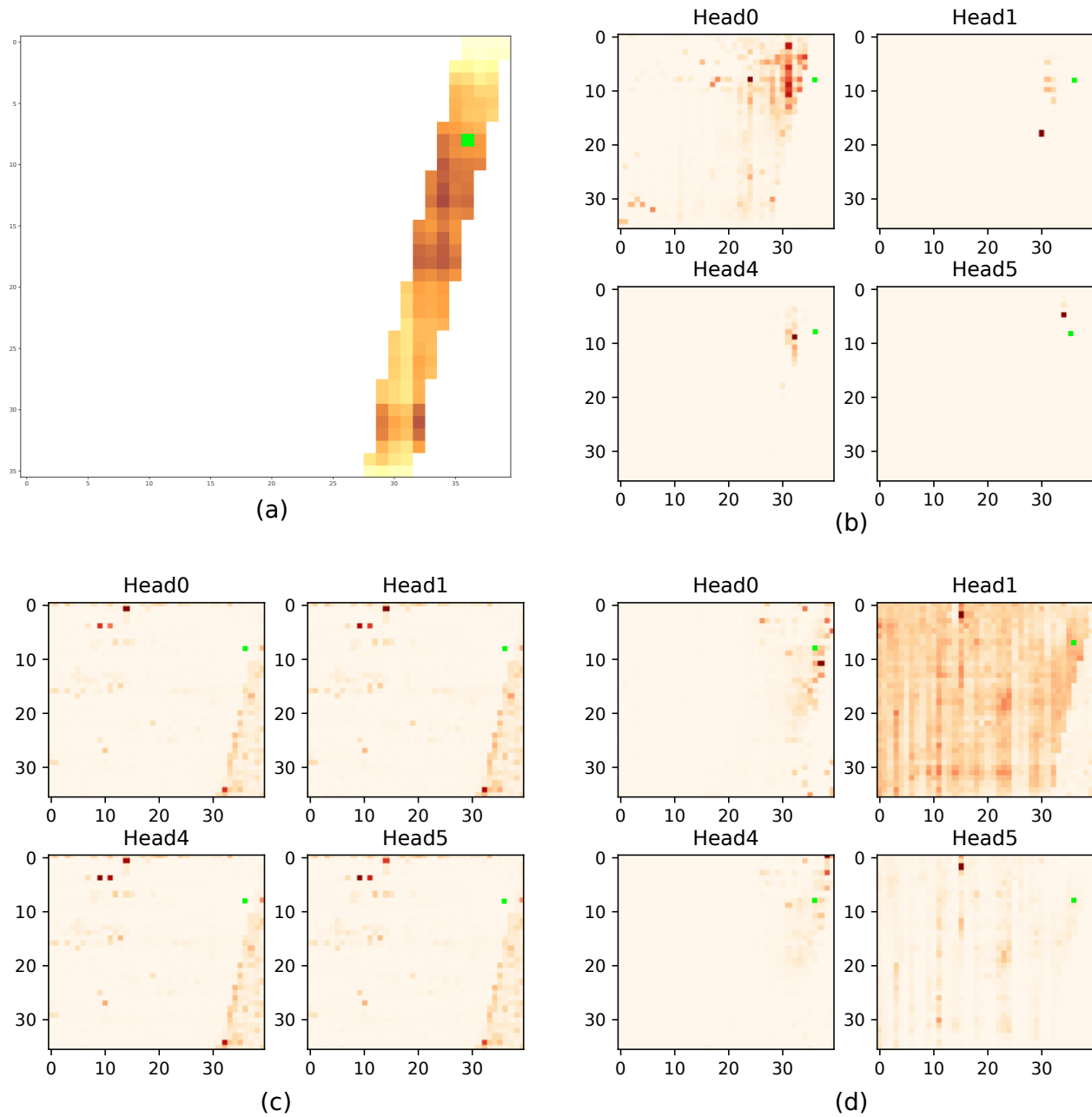
FIGURE 7: Visualisation of attention scores of 4 heads for a single pixel from the Channel Vision Transformer: (a) Studied I(t) with the targeted pixel; (b) Attention scores from the passenger load channel; (c) Attention scores from the travel time channel; (d) Attention scores from the waiting time channel; [A deeper red color indicates a higher attention score]
