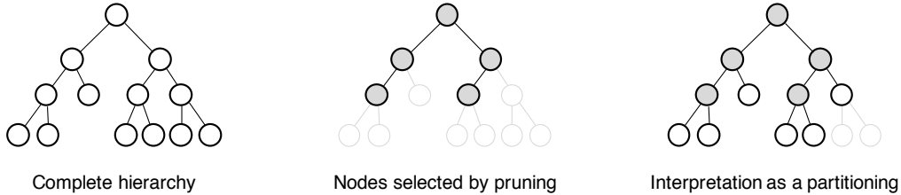
Figure 7: Left: Example of a complete generalisation hierarchy. Middle: Example of a pruning of the hierarchy, satisfying the tree constraint. Right: Interpretation of the pruning as a partitioning of the values.
