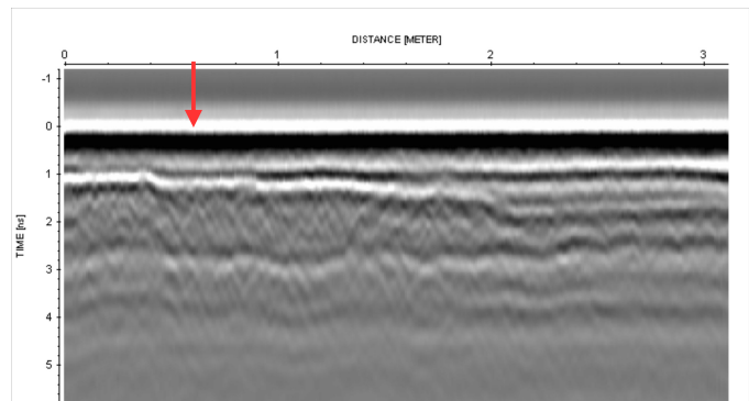
Fig. 10. GPR B-scan, done on Line 6 at the series T4 (22' of imbibition)
