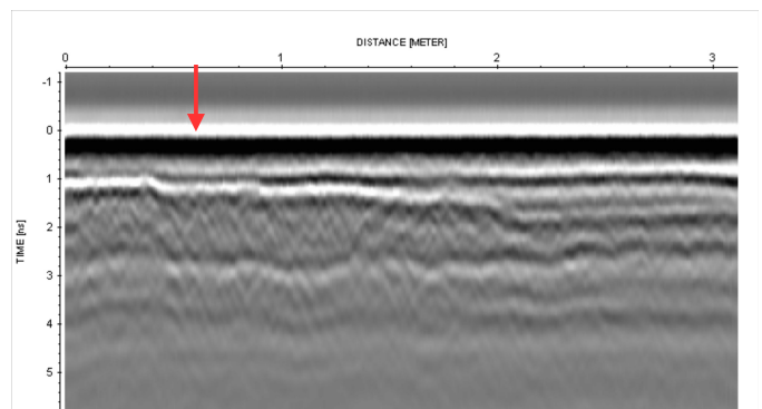
Fig. 10. GPR B-scan, done on Line 6 at the series T4 (22' of imbibtion)
