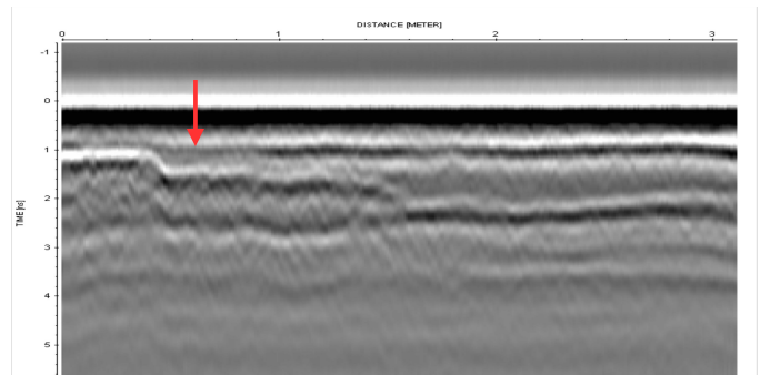
Fig. 9. GPR B-scan, done on Line6 at the series T3 (16' of imbibtion). The red arrow shows the location of the SFR measurements
