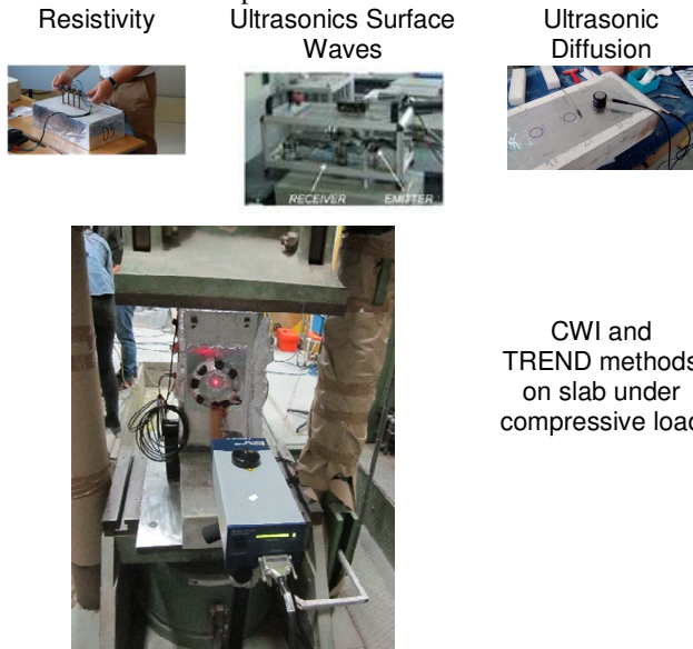
FIGURE 1: EXAMPLES OF NDE METHODS APPLIED ON LABORATORY SLABS
