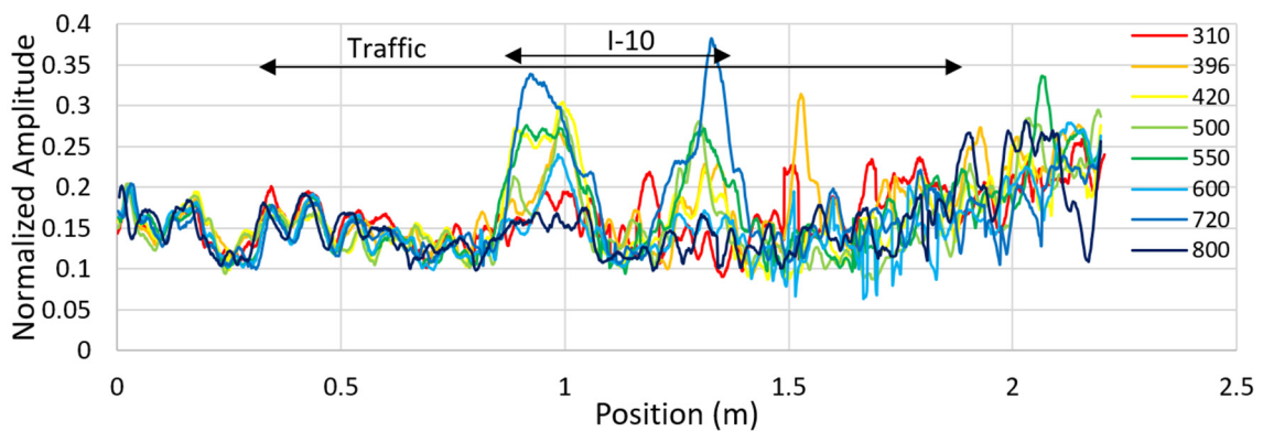
Figure 38. 2.6 GHz Normalized RW amplitudes on defect I-10, in the transversal direction vs. K loadings.
