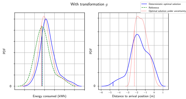
Figure 10: Normalized PDFs of the consumed energy (left) and of the distance to arrival position (right) for the transformed optimal solution of the deterministic problem g(u^{\text{mode}}, \mathbf{Z}_f) (in blue), the family of optimal solutions of the deterministic problems u^{(1)}, \dots, u^{(M)} (in green), and the transformed optimal solution under uncertainty g(u_K(\cdot; \alpha^*); \mathbf{Z}_f) (in red) empirically estimated from realizations z^{(1)}, \dots, z^{(M)} of \mathbf{Z} . z^{\text{mode}} is represented with a vertical dotted line.
