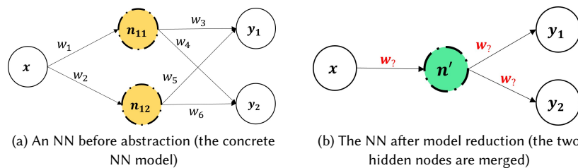
Fig. 6. Model reduction of a small neural network
