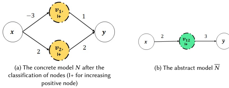
Fig. 8. Counterexample of Elboher et al. [16] abstraction method
