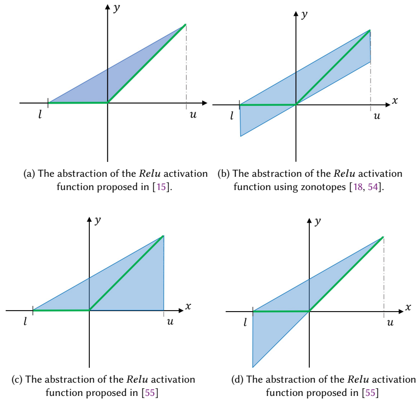
Fig. 5. Relu activation function abstractions using different abstract domains. The Relu ( y = \text{relu}(x) ) is represented by the green line and its over-approximation on the range x \in [l, u] by the blue filled area.
