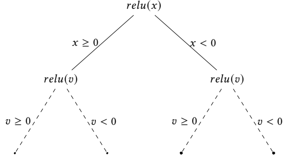
Fig. 3. An example of state-space explosion. For two Relu nodes, case splitting leads to four linear subproblems.
