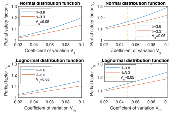
Figure 3: Influence of the distribution type for steel and concrete
