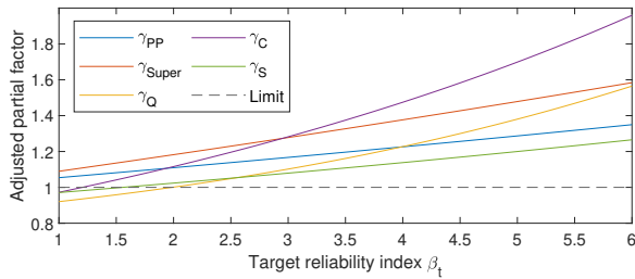
Figure 2: Influence of the target reliability index on partial factors
