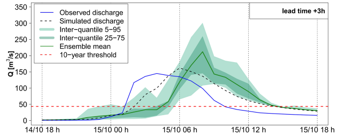
Figure C3. Detailed hydrograph for 3 h lead time forecast evaluation at outlet 3 for AROME-EPS. In blue, the observed discharge at the gauging station.
