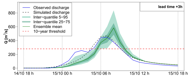
Figure C5. Detailed hydrograph for 3 h lead time forecast evaluation at outlet 5 for AROME-EPS. In blue, the observed discharge at the gauging station.
