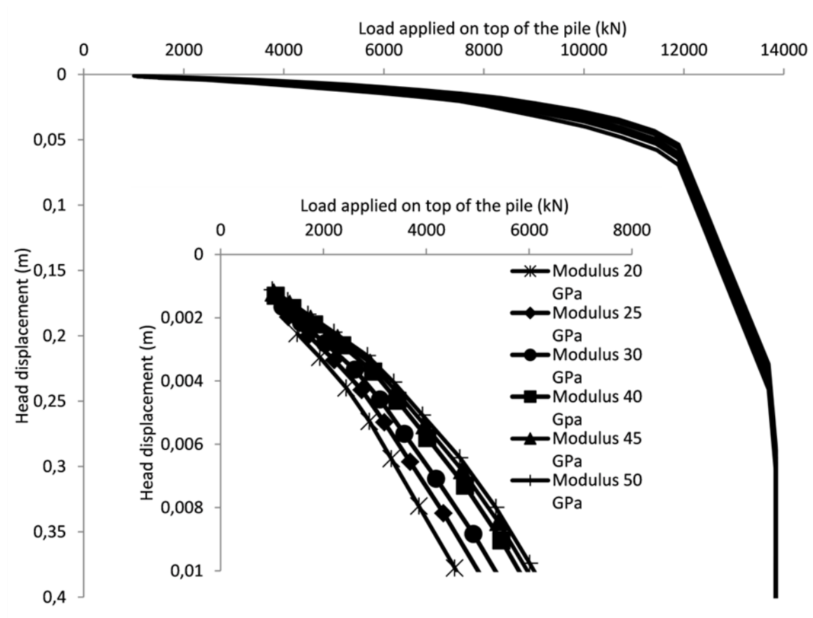
Fig. 1 Load-settlement curves for a same pile with different modulus (with a focus on the first part of the curve)
