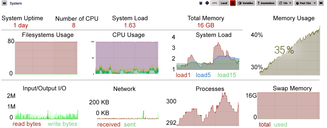
Fig. 2. Physical Machine Metrics Evolution over Time
