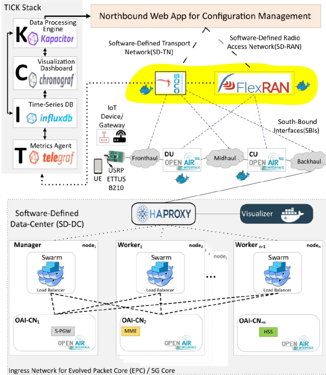
Fig. 1. Experimental Prototype Architecture
