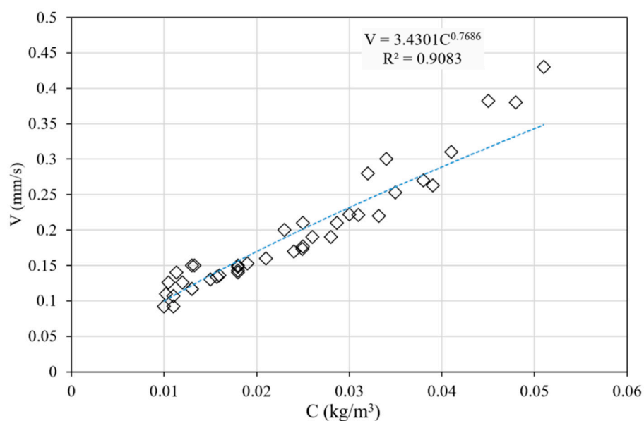
Figure 5. Variation of the settling velocity with SSC on the Lobo reservoir.
