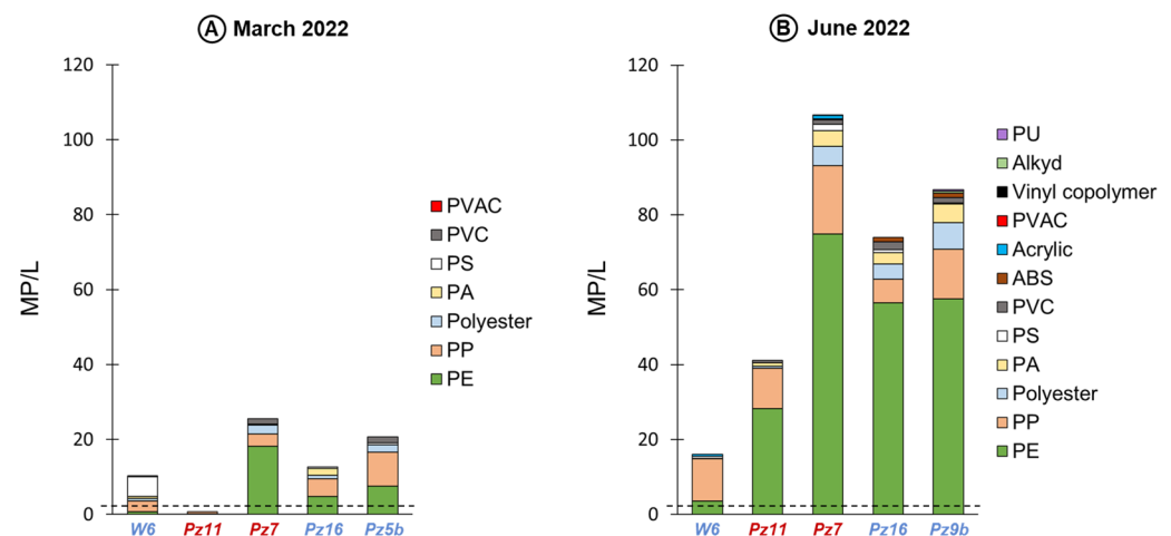
Figure 5. MP concentrations (in MP/L, MP > 25 μm, the dotted black lines indicate field blank concentrations) and polymer types at the different sampling points in (A) March and (B) June 2022. Wells and piezometers catching the alluvial groundwater from upstream to downstream are represented in blue, piezometers catching the landfill groundwater are represented in red.
