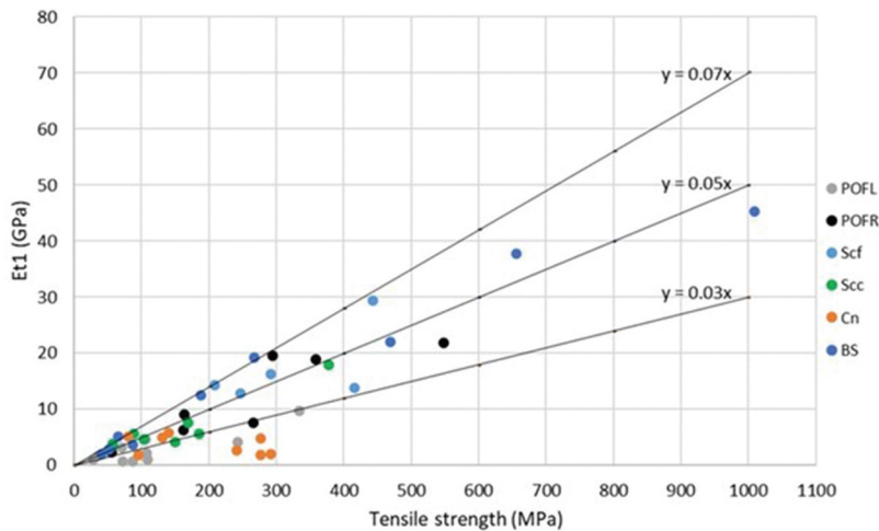
Figure 8. Modulus of elasticity vs tensile strength.
