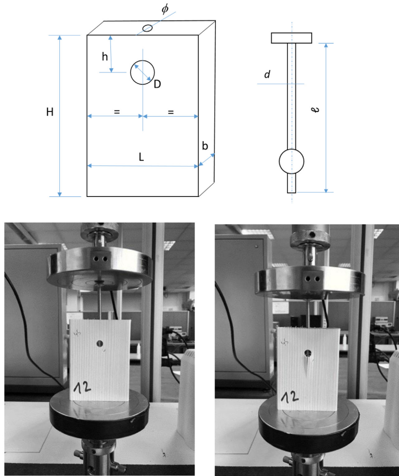
Fig. 2. (Top left) Geometry of the spruce specimens containing a horizontally centered circular through hole with diameter D and depth b (corresponding to the specimen depth), and a top circular non-through hole with diameter \phi and a depth of 55 mm. (Top right) Geometry of the screw with length \ell and diameter d . (Bottom) Example of compression test performed on sample #12.
