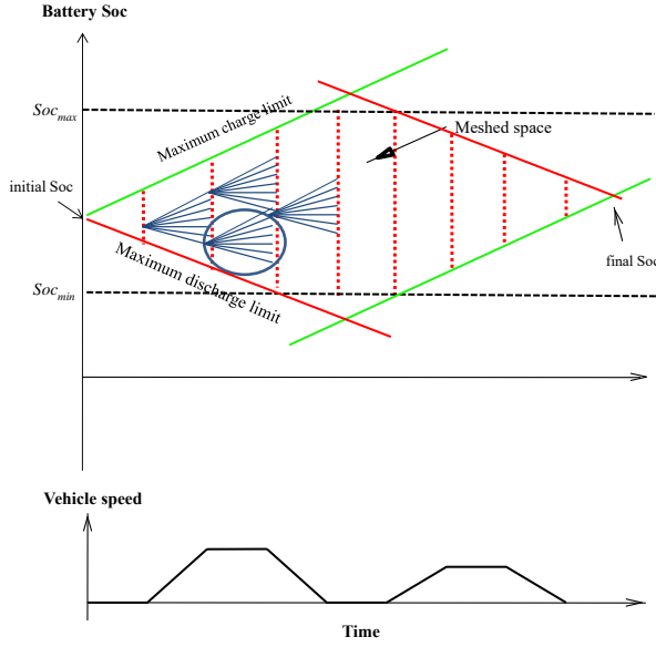
Figure 7: Mesh of the battery state of charge domain for the dynamic programming method
