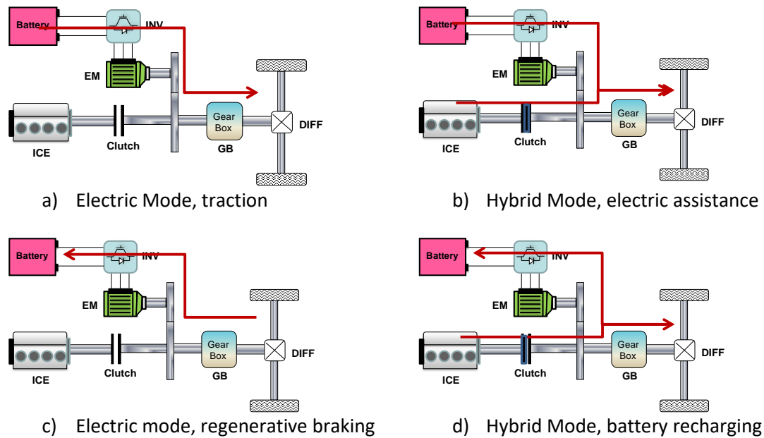
Figure 2: Examples of operating modes encountered in a parallel HEV
