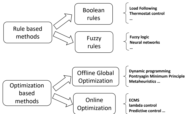
Figure 4: Energy Management Strategies classification
