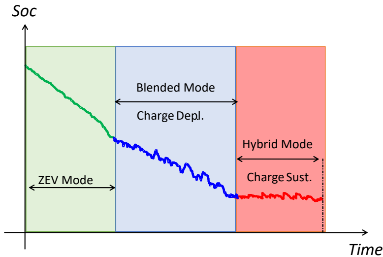
Figure 3: Soc battery control possibilities in an HEV
