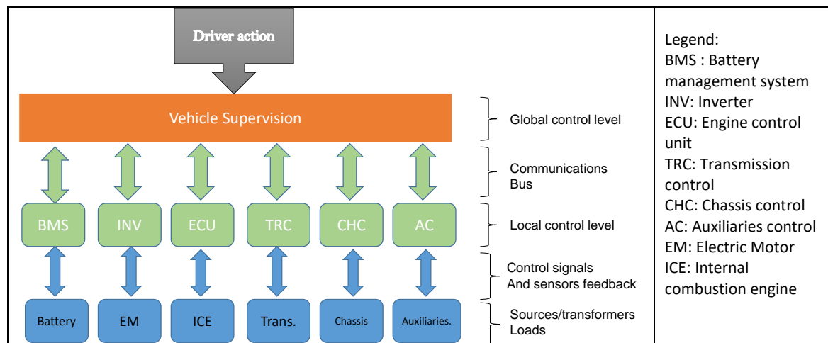
Figure 1: HEV control levels
