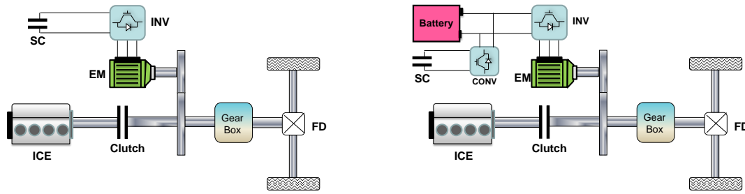
Figure 9: Example of parallel HEV with SC as ESS Figure 10: Example of parallel HEV with hybrid ESS (battery and SC)
