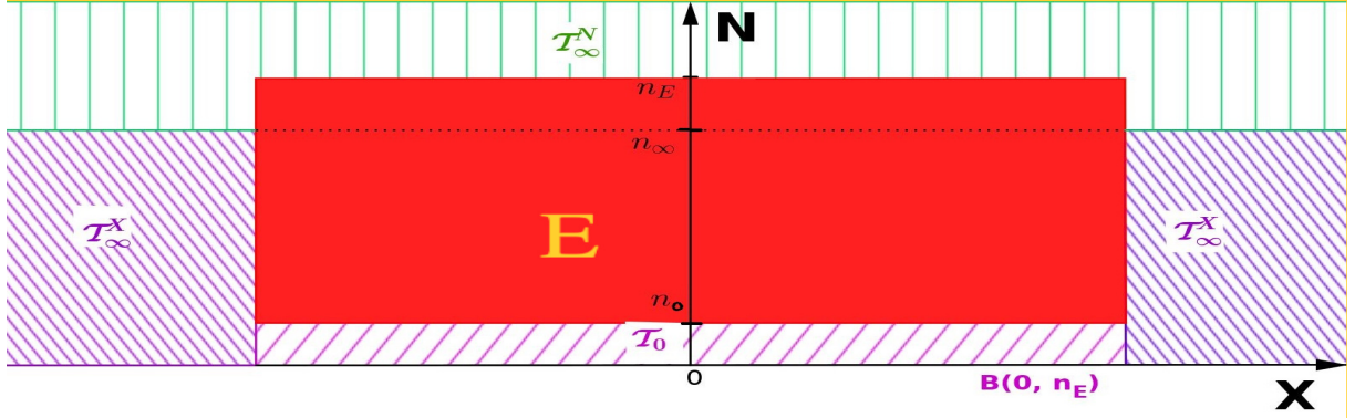
Figure 1: subdomains for (A2)
