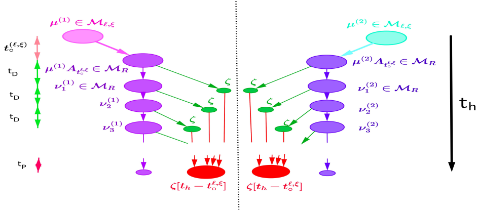
Figure 2: Illustration of the coupling procedure
